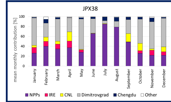
Mean monthly contribution of Xe-133 emissions from individual sources as observed at IMS stations. The results are based on operationally produced ATM results (backward modelling) using meteorological data from ECMWF.
