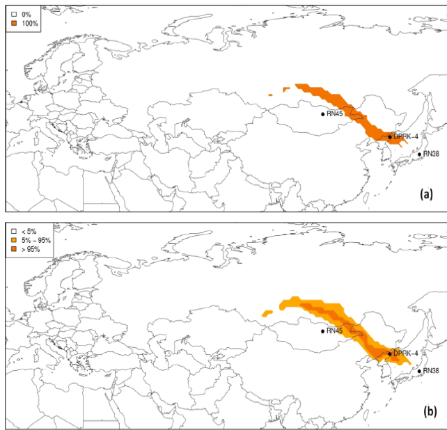
Figure 3. Pointwise probability that a certain grid point is a possible source for (a) the unperturbed simulation (thus fully deterministic) and (b) the full 51 member ensemble. Maps have been generated using ref. 48.
