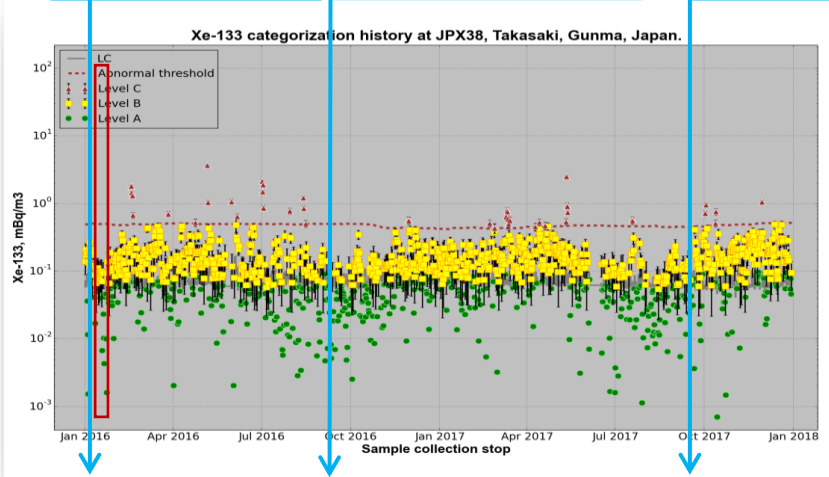
Xe-133 Categorization History
