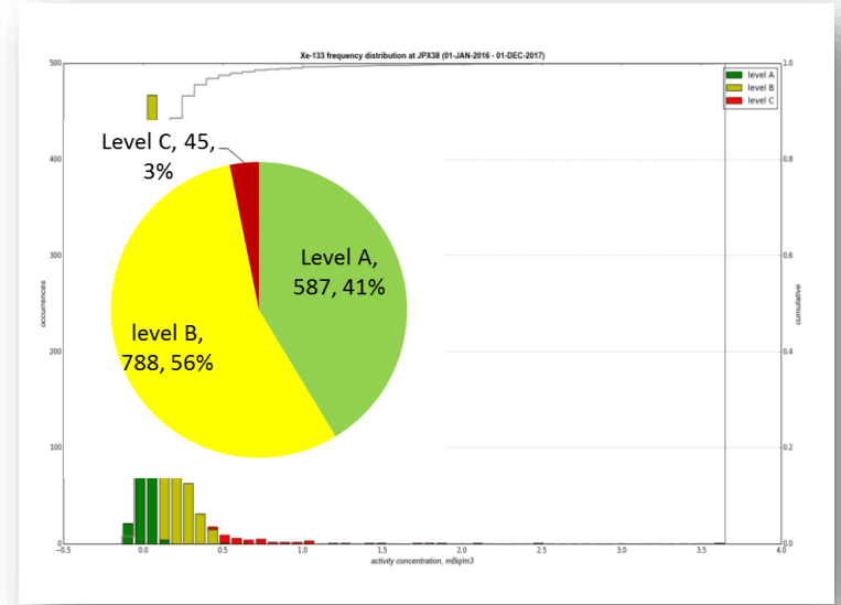
Xe-133 Frequency Distribution
